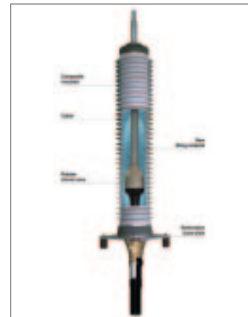
Terminale oil-free.
